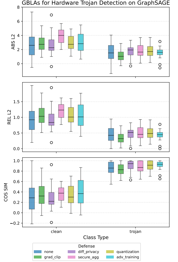
Fig. 5: Hardware Trojan Detection: Reconstruction errors under different defense mechanism for GraphSAGE.
