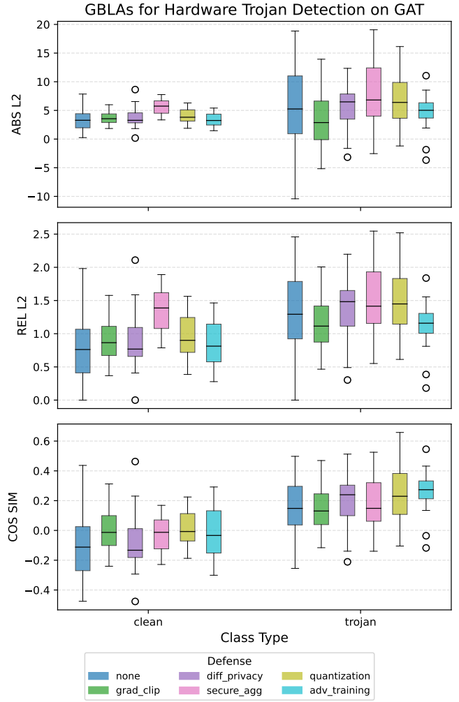
Fig. 7: Hardware Trojan Detection: Reconstruction errors under different defense mechanism for GAT.
