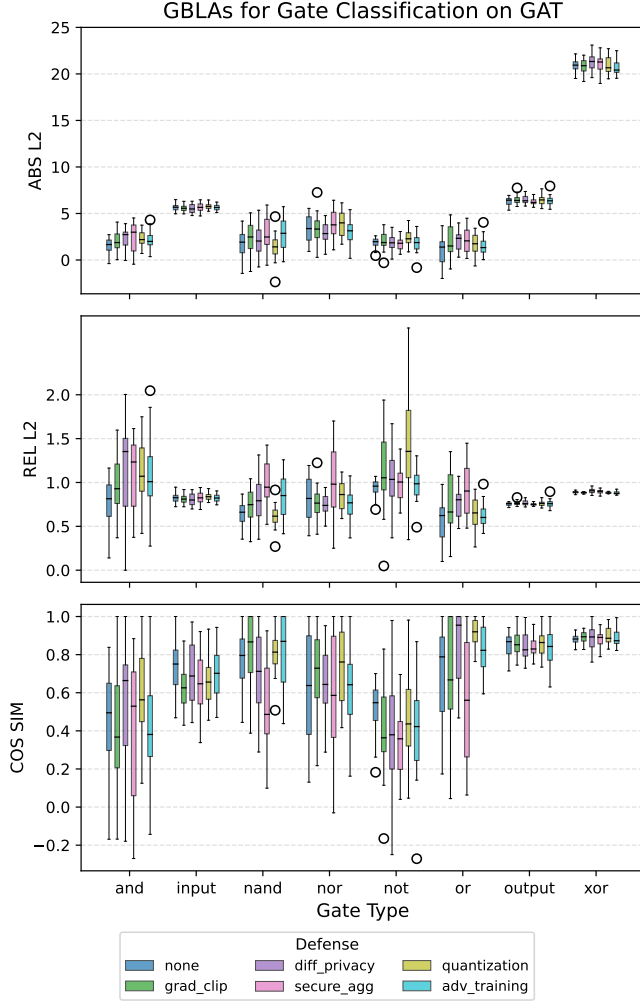
Fig. 4: Gate Classification: Reconstruction errors under different defense mechanism for GAT.
