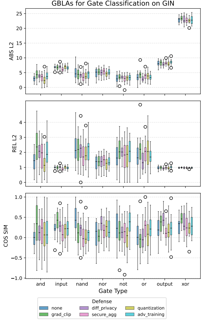
Fig. 3: Gate Classification: Reconstruction errors under different defense mechanism for GIN.
