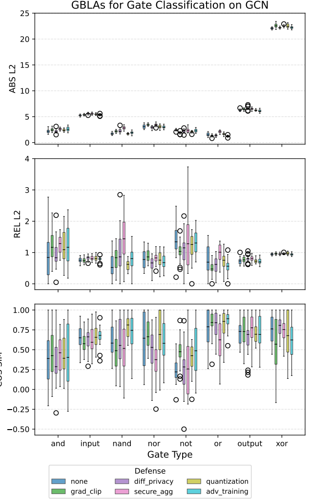
Fig. 1: Gate Classification: Reconstruction errors under different defense mechanism for GCN.
