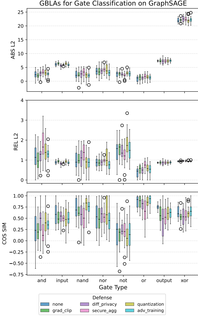
Fig. 2: Gate Classification: Reconstruction errors under different defense mechanism for GraphSAGE.
