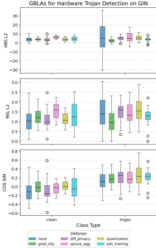
Fig. 6: Hardware Trojan Detection: Reconstruction errors under different defense mechanism for GIN.
